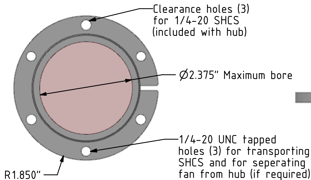
Aluminum EZE-Hub® Part# 3-00
