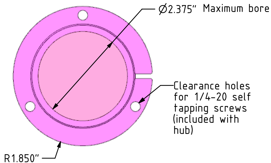
Aluminum EZE-Hub® Part# 3-00
